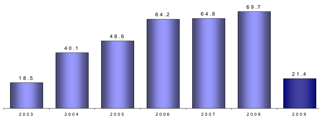
Chart 2. Inflow of FDI to the new EU member states in 2003-2009 (USD billion)
