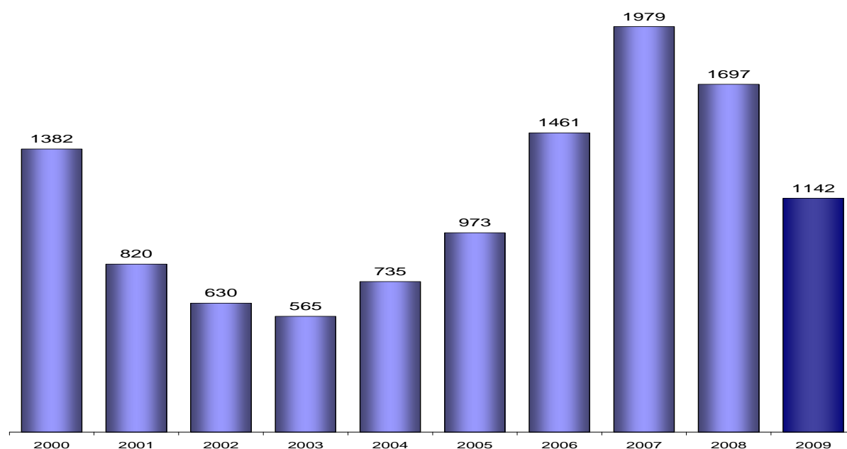
Chart 1. FDI worldwide 2000-2009 (USD billion)
